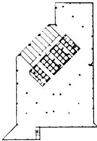
⑤ Typical floor, plinth area, 101 Park Avenue, New York City (48 storeys)
